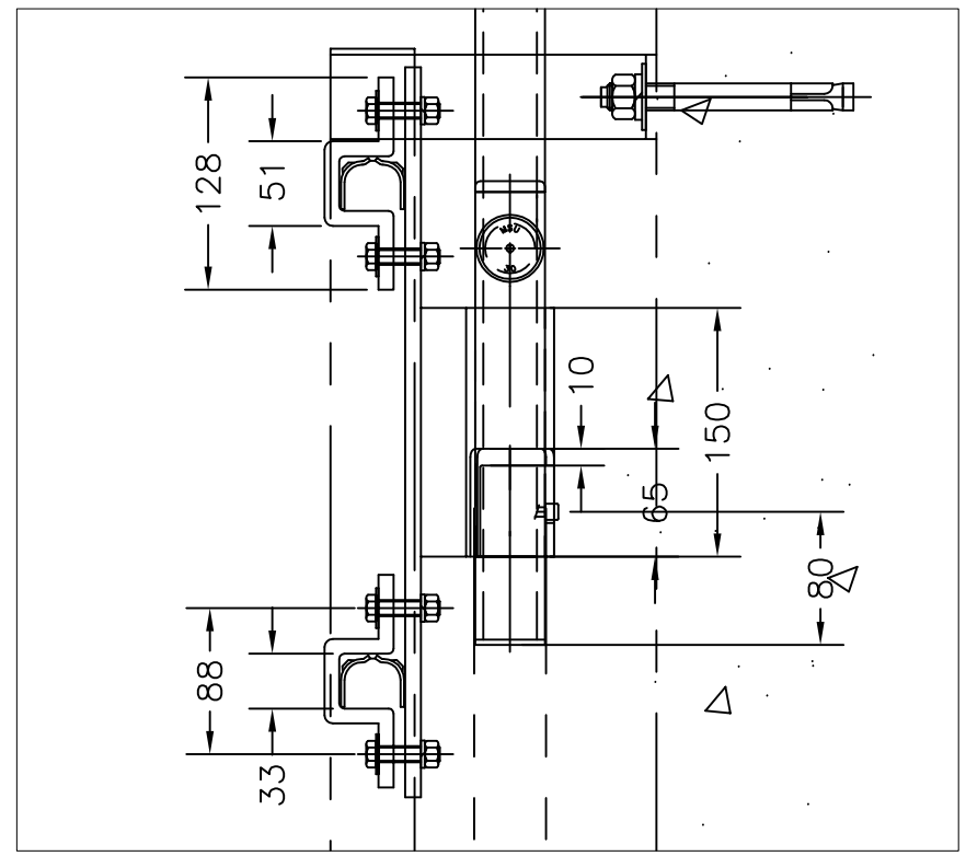
SOCKET DETAIL
